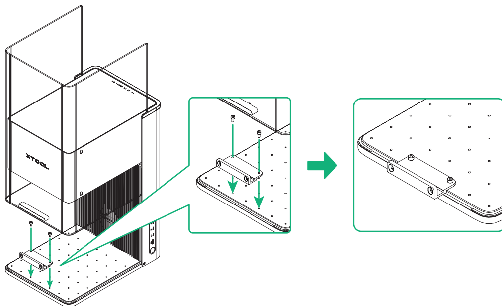
Fastening piece A
