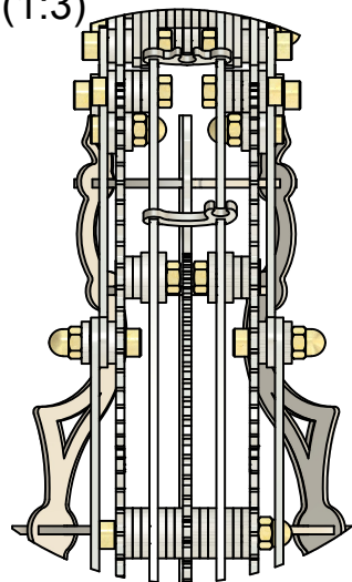
D (1:3)
